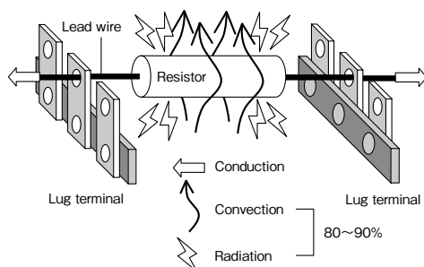
【Figure 2. Heat dissipation of cylindrical resistors】
