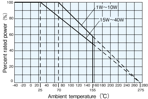
■ Derating Curve
