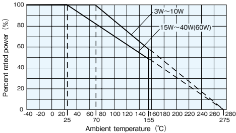
■Derating Curve
