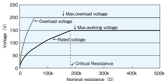
【Example of various voltage of RK73G 2A】
