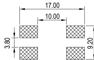
( PCB Pattern )
