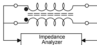
Measuring Circuit:
