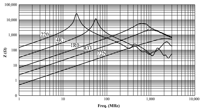
Z vs Freq Plot
