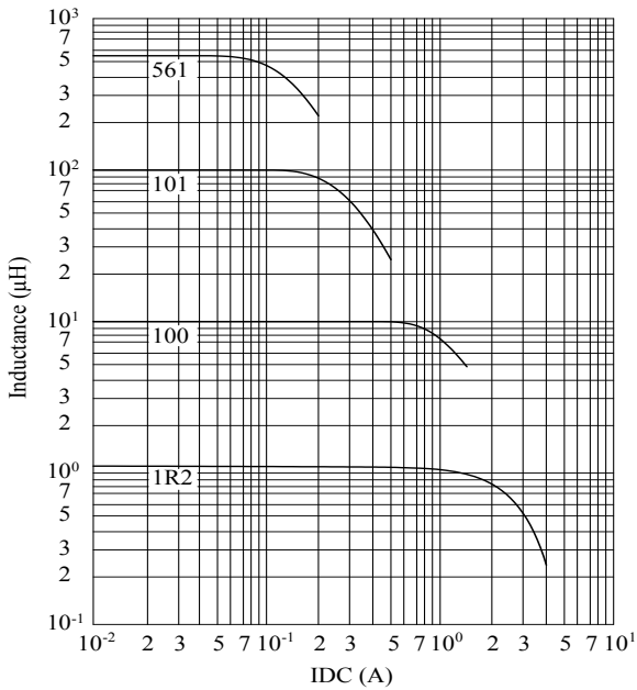
@ Inductance VS. DC Current Curve
