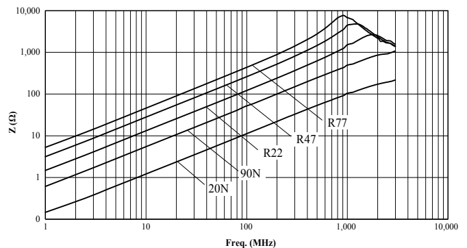
Z vs Freq Plot
